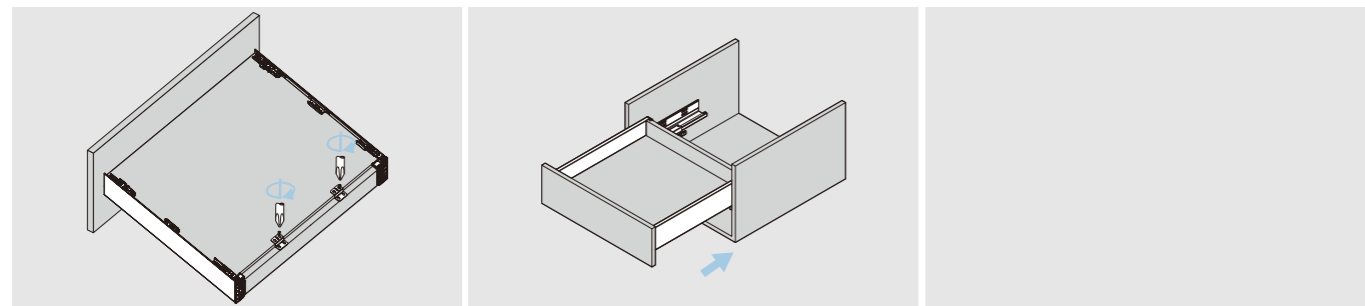
Fixing-brackets assembly
