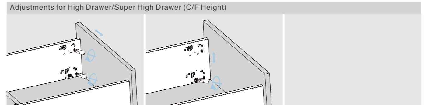
Left&right adjustment
